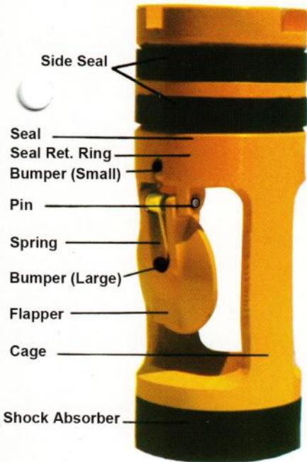
Flapper Type
